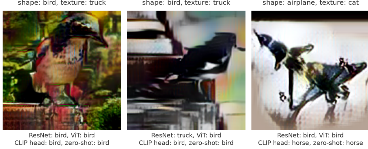
Figure 1: Example Images
