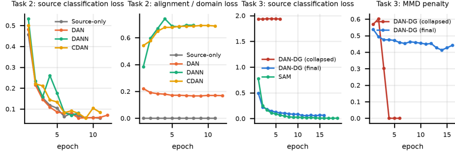
Figure 4: Training curves
